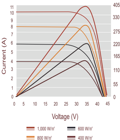
I-V Curves at Different Irradiances (400W) Test Temperature: 25°C
