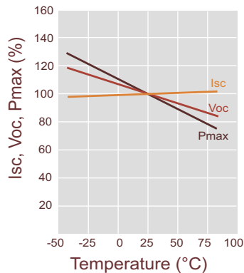
Irradiance: AM 1.5, 1,000W/m 2 ( 450W)
