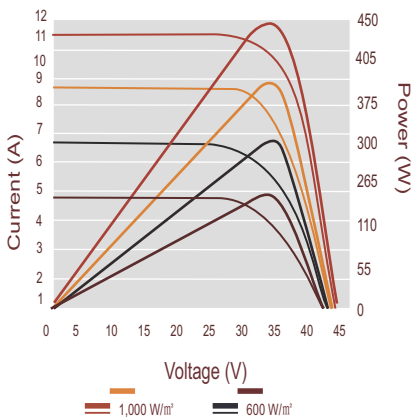
I-V Curves at Different Irradiances (450W) Test Temperature: 25°C
